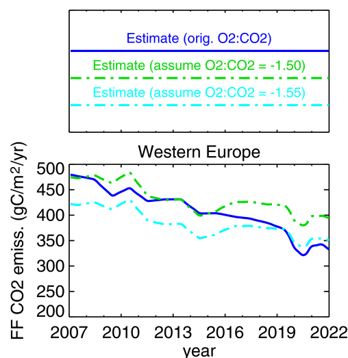
Figure 6. Importance of the O 2 : CO 2 stoichiometry of FF emissions ( \alpha_{\text{FF,pri}} ) used in the APO inversion: a given FF CO 2 emissions estimate based on the original time and space varying \alpha_{\text{FF,pri}} from the bottom-up inventory (blue, here using the FF inventory as a proxy for an inversion result) is compared to CO 2 emissions re-computed from the corresponding APO flux assuming constant stoichiometries of −1.50 (green) or −1.55 (cyan), respectively.
