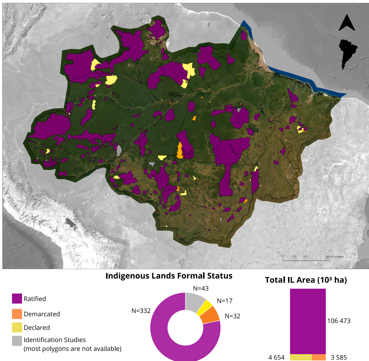
Fig. 1. Formal stages of Indigenous Land demarcation across the Legal Brazilian Amazon. Map of Indigenous Lands (ILs) showing the formal stages of demarcation reached for 381 ILs for which boundary polygons are available. Most of the 43 ILs at Stage 1 of the administrative process have not been physically delimited nor have an official polygon and therefore are not shown.
