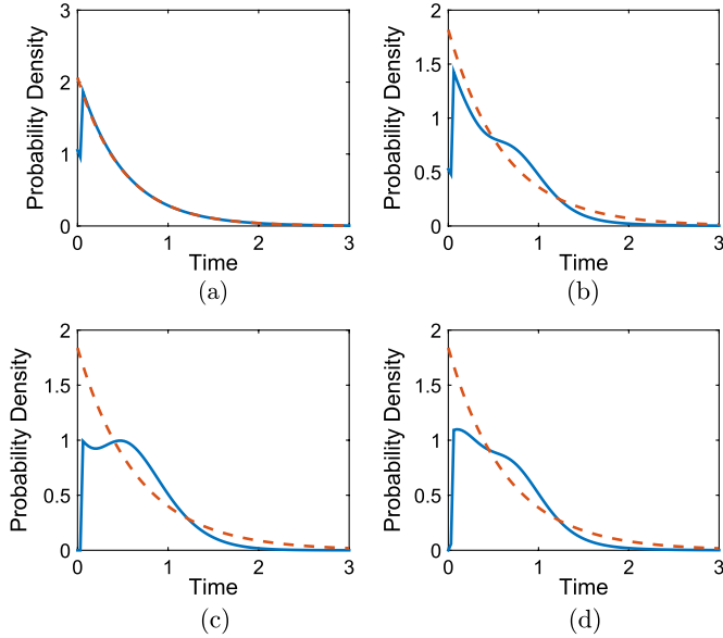
Fig. 5. PDF of handoff session eCHT (solid line) and its exponential fitting (dashed line) when CRT is hyper-Erlang distributed with two parameters (m_1, m_2, \eta) . (a) m_1=1, m_2=1 . (b) m_1=1, m_2=10 . (c) m_1=5, m_2=5 . (d) m_1=2, m_2=10 .
